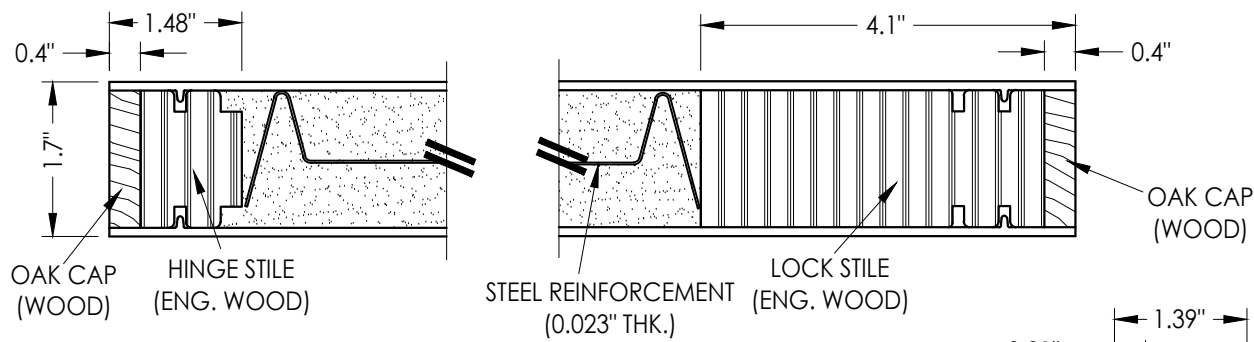
1 HORIZONTAL CROSS SECTION
