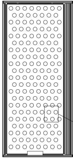
DOOR PANEL SECTION PANEL REINFORCEMENT (0.023" Thick Steel) STEEL REINFORCEMENT 28.86% OPEN AREA MAX.
